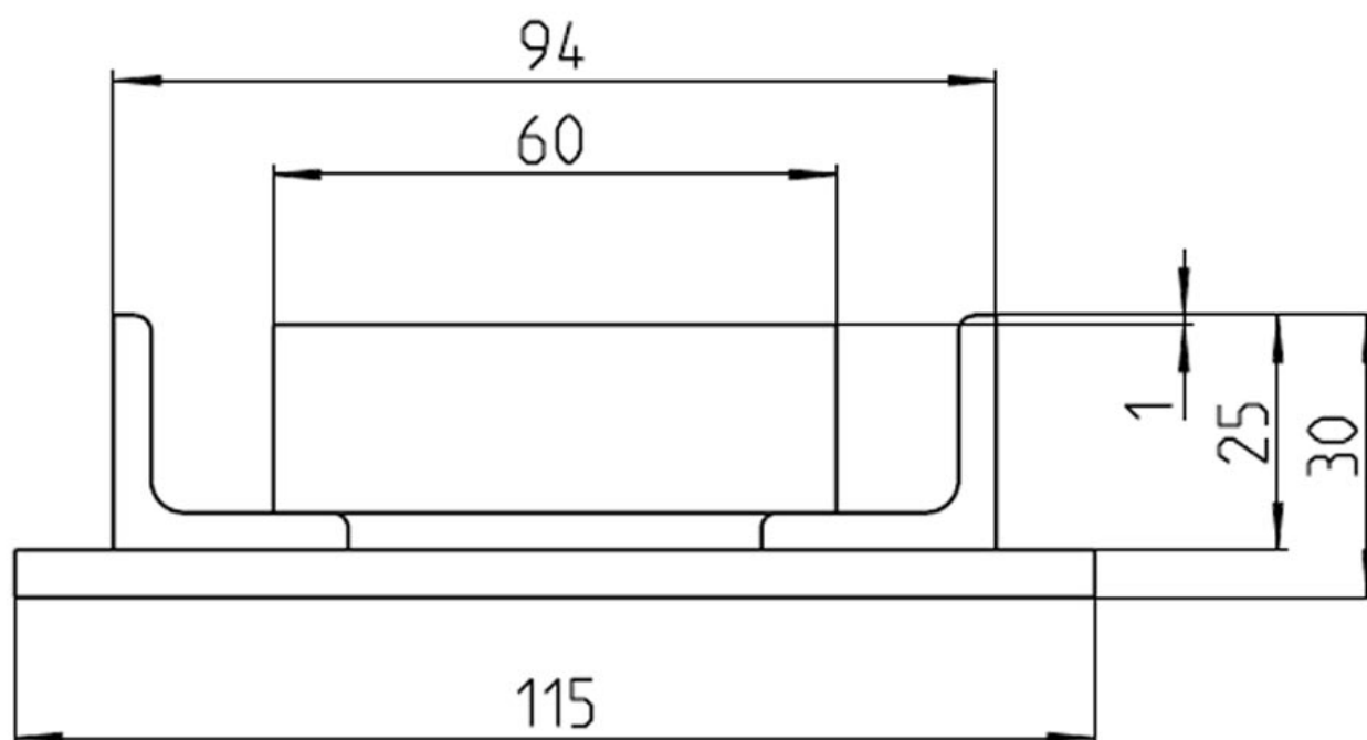
Technical drawing RS-2-FG
