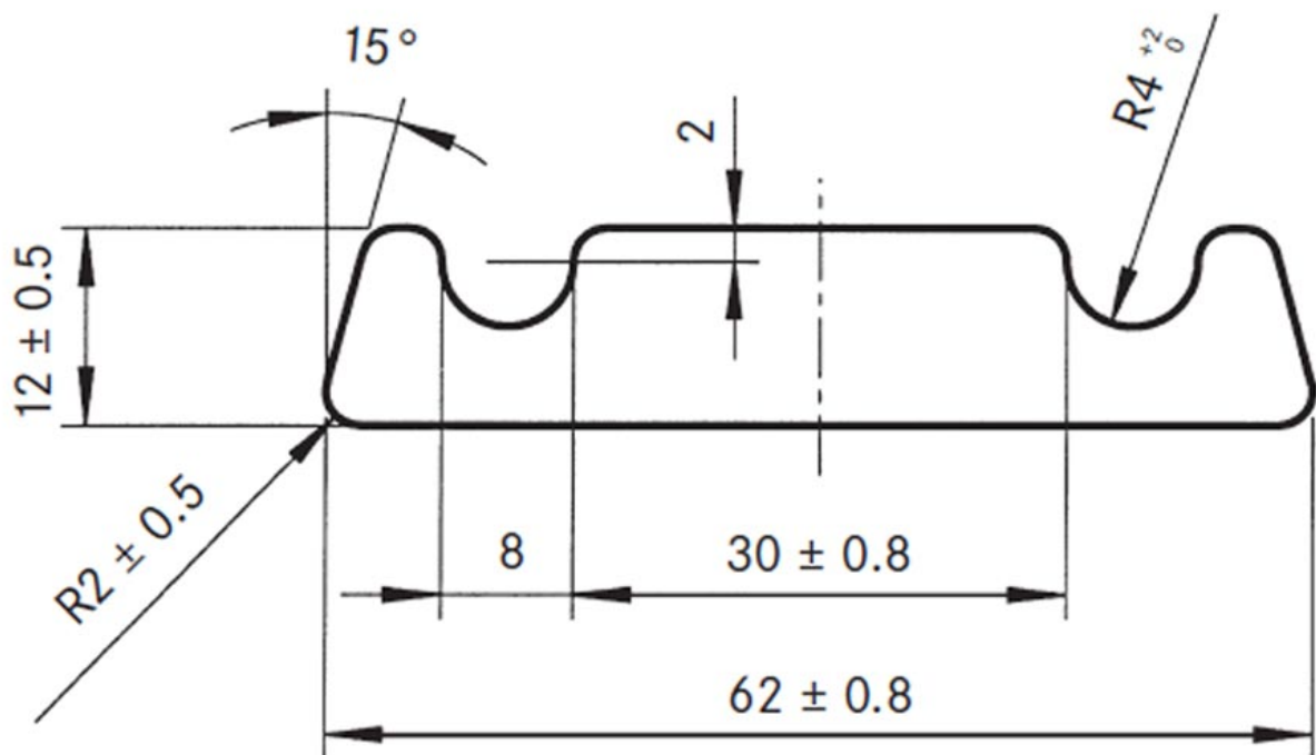
Technical drawing RS-1
