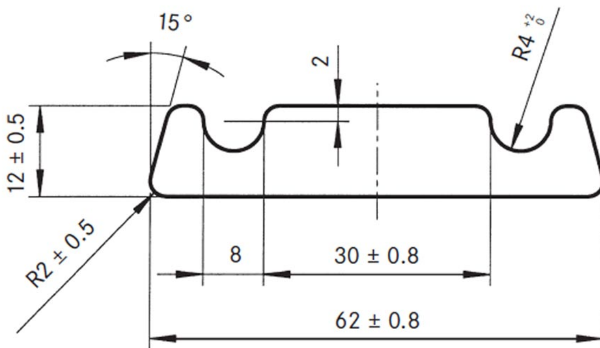
Dessin technique RS-1
