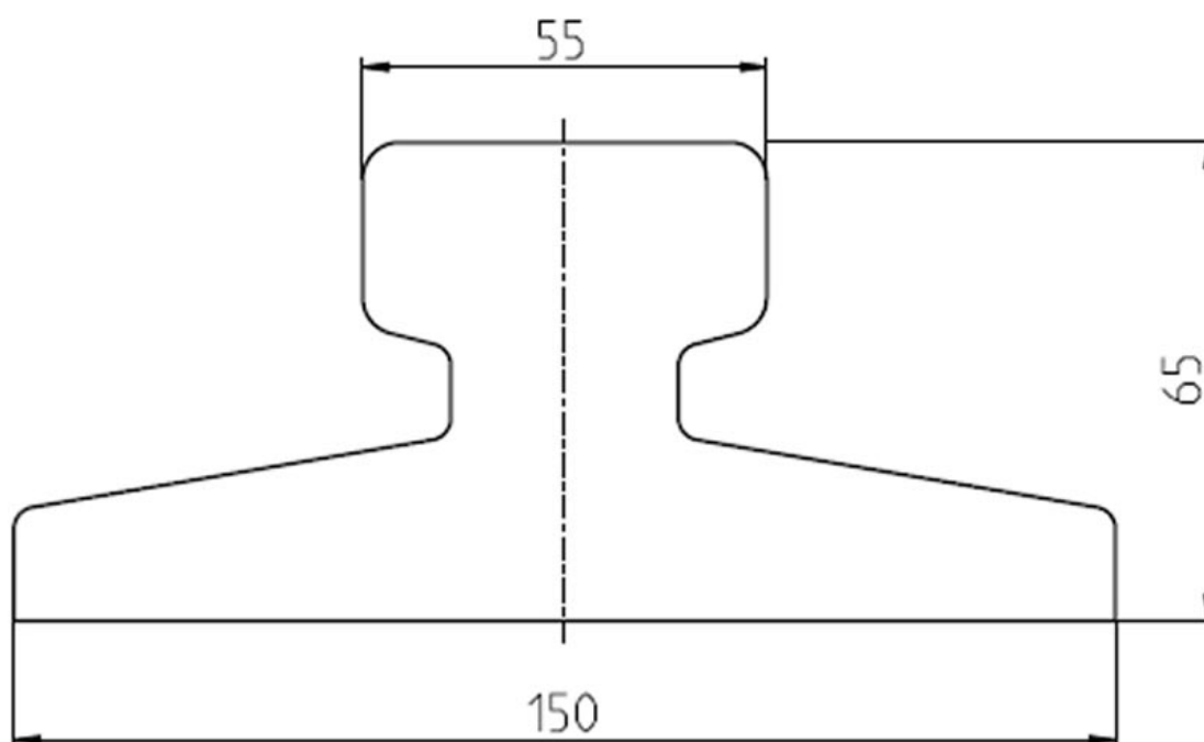
Technical drawing W-55
