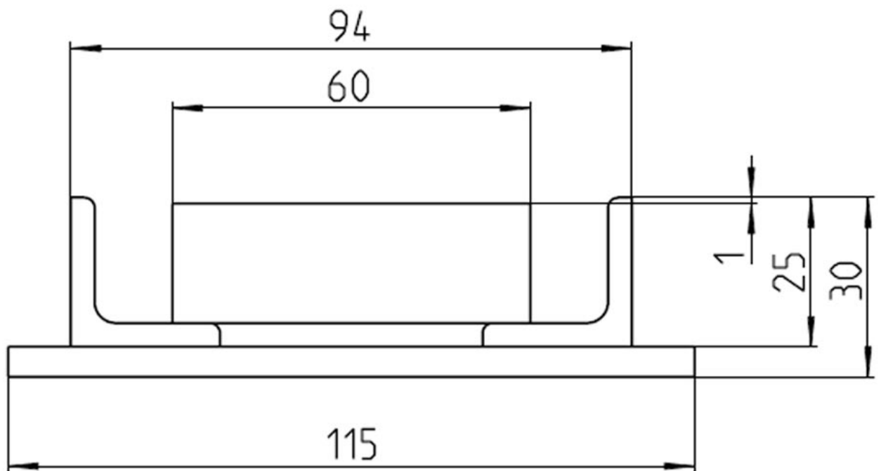
Technical drawing RS-2-FG
